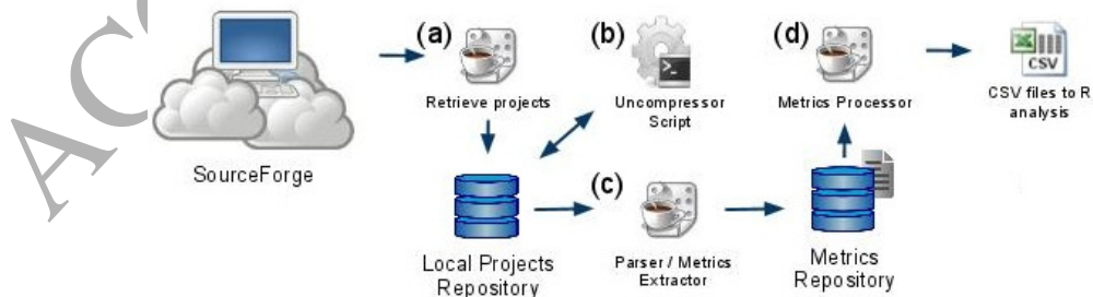
Figure 1: In (a) the crawler populates the infrastructures repository with Java Projects from Sourceforge. In (b) a shell script extracts all compressed files into our local repository. In (c) the metrics collection tool parses the source code, collects metrics, and stores the results in the metrics repository. In (d) the metric collection tool generates input CSV files to be statistically analyzed by R.
